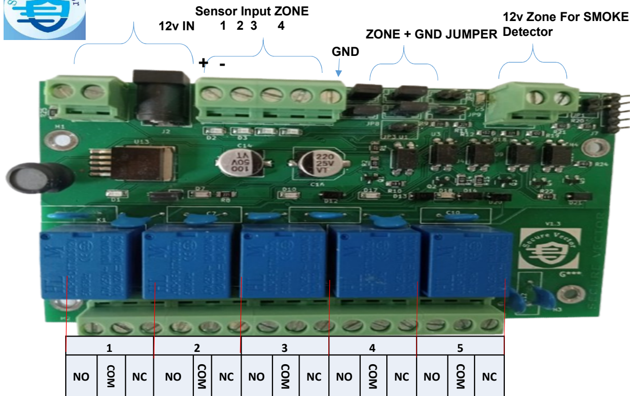
5 RELAY NO / NC CONNECTION
